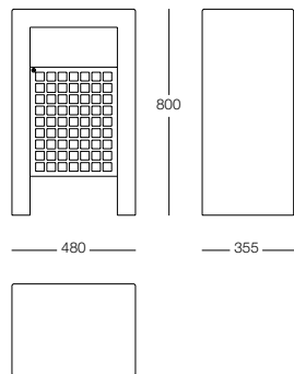
steel and wood litter bin 35L corbeille en acier et bois 35L papeleira em chapa e madeira 35L
